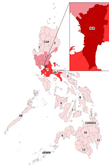
Fig. 2: Proportion of newly diagnosed cases by region of residence, Jan-Mar 2020 (N=2,818)
