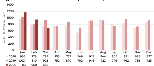
Fig. 3: Number of ART initiation per month, 2018-2020
