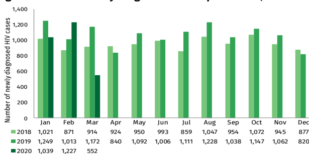
Fig. 1: Number of newly diagnosed cases per month, 2018-2020
